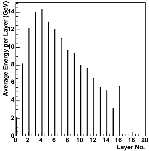
150 GeV Pion, Int. in HB
