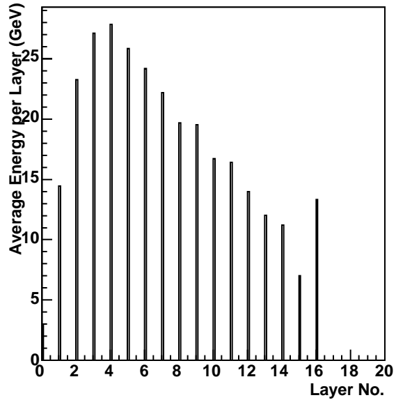
300 GeV Pion, Int. in HB
