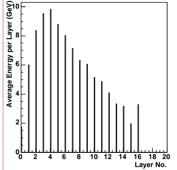
100 GeV Pion, Int. in HB
