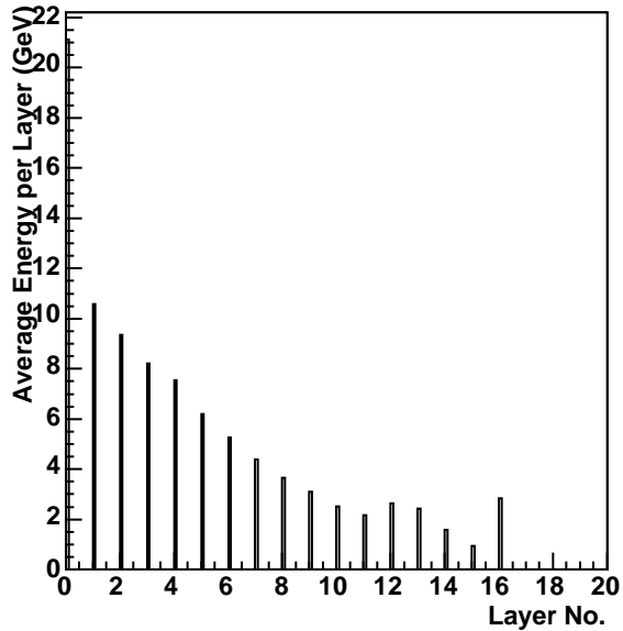
150 GeV Pion, Int. in ECAL
