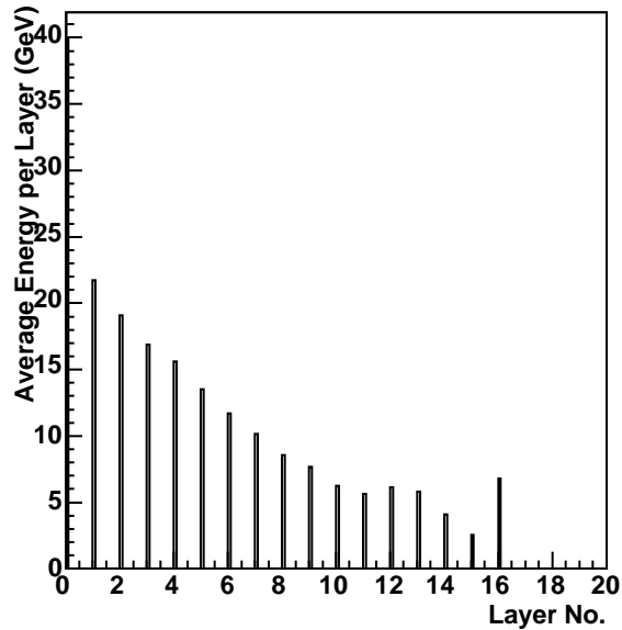
300 GeV Pion, Int. in ECAL
