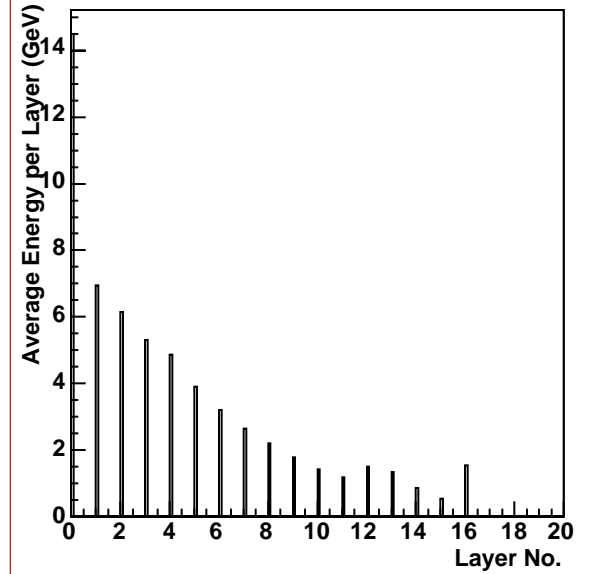
100 GeV Pion, Int. in ECAL
