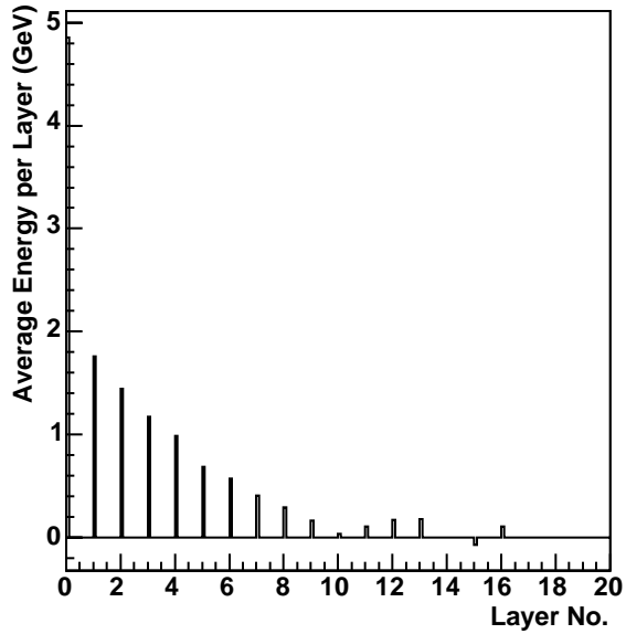
30 GeV Pion, Int. in ECAL
