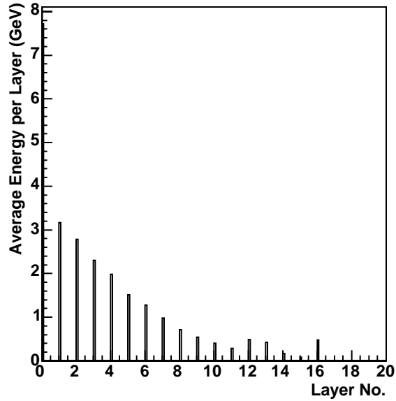
50 GeV Pion, Int. in ECAL
